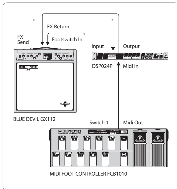
Fig. 3.2: Guitar setup (using the switch function)
